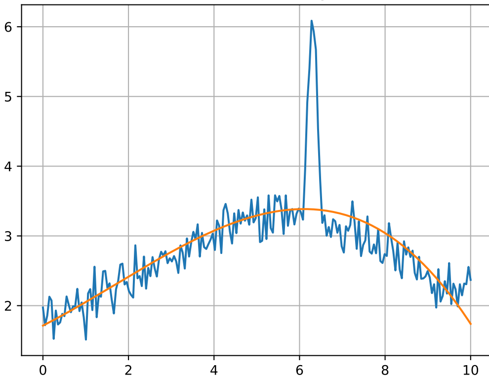
Continuum Fitting
